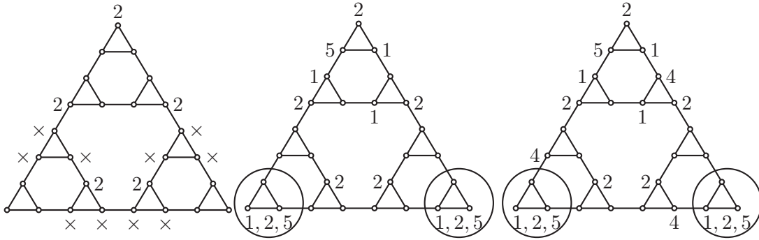
Figure 3: Partial 6-packing coloring(s) of S^3 when |c^{-1}(2)| = 7
