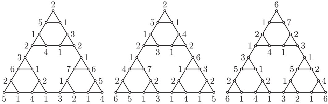
Figure 7: Colorings of types C_{6,2} , C_{6,1} , and C_{5,2}
