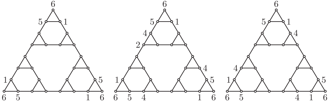
Figure 4: Partial 6-packing coloring(s) of S^3 when |c^{-1}(2)| = 6
