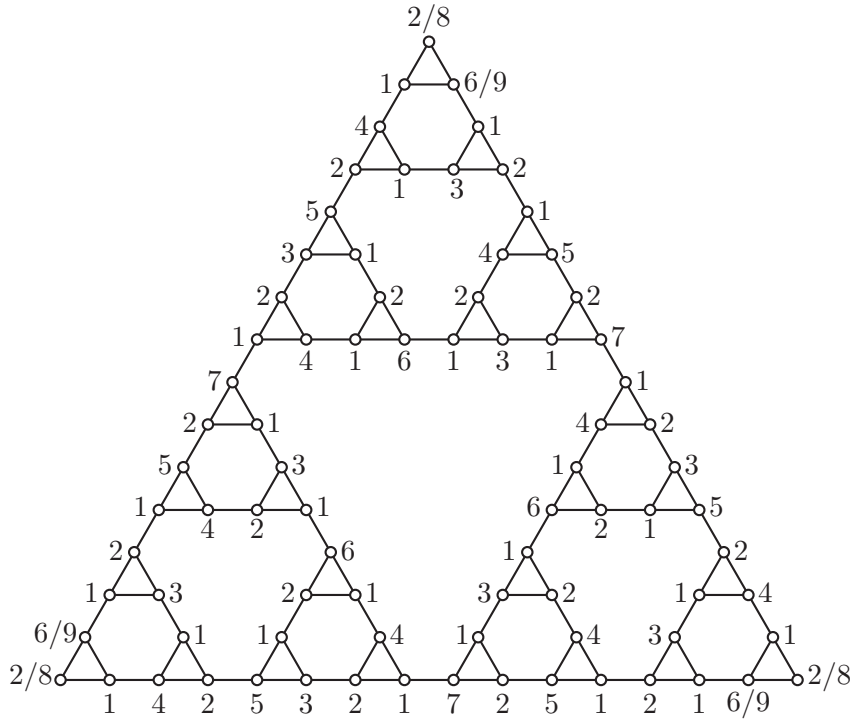
Figure 5: Packing coloring(s) of S^4
