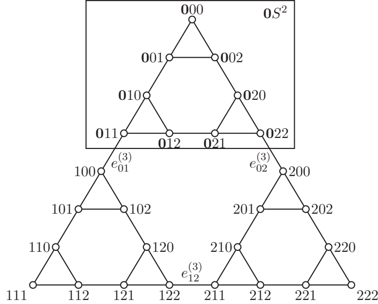
Figure 1: The Sierpiński graph S^3
