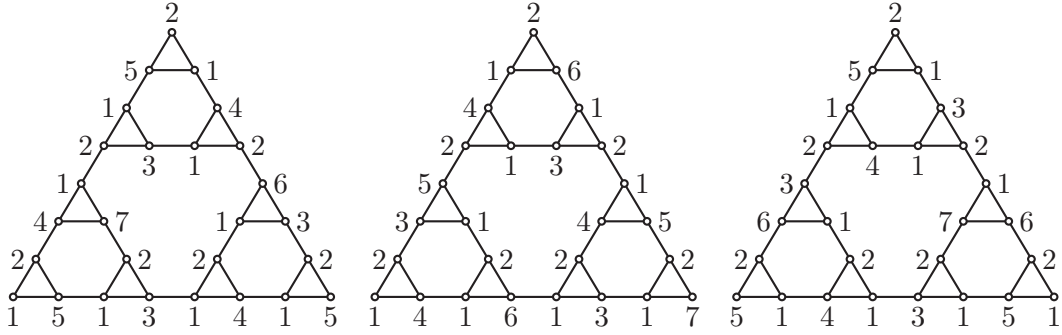
Figure 6: Colorings of types C_{6,6} , C_{6,5} , and C_{6,4}
