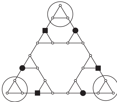
Figure 2: Partial packing coloring with |c^{-1}(4)| = 3
