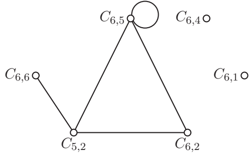
Figure 8: The relation graph of the remaining compatible types of 7-packing colorings of S^3
